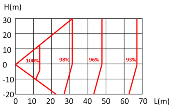
Figure 2-7.10: 60 model rate of change in heating capacity
