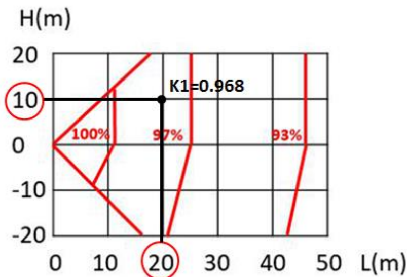
Figure 1-5.4: Ultima rate of change in cooling capacity
