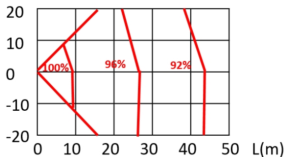
Figure 2-7.8: 48/56 model rate of change in heating capacity
