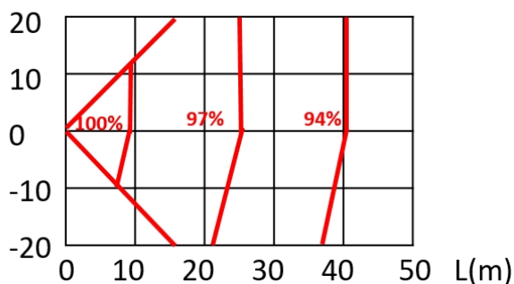
Figure 2-7.7: 48/56 model rate of change in cooling capacity
