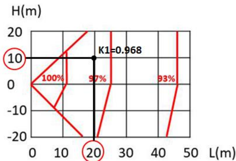
Figure 1-5.3: Ultima rate of change in cooling capacity
