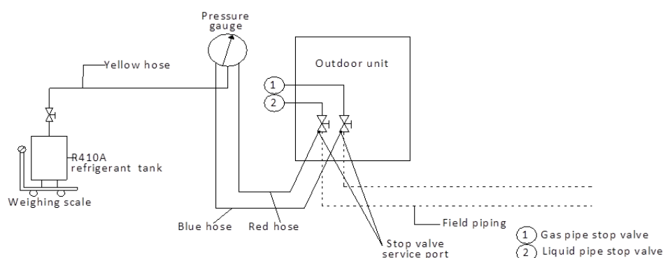
Figure 3-4.12: Vacuum drying
