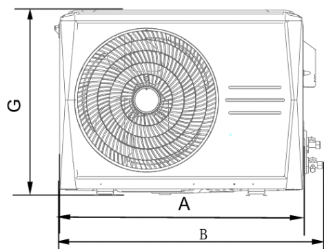
Figure 2-2.1: Model 28-36 Front view dimensions
